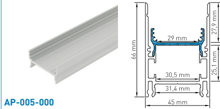
AP-005-000 Aluminium Einsatz MF Aluminium inset MF
